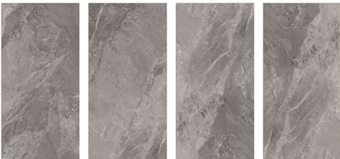
Random Design
