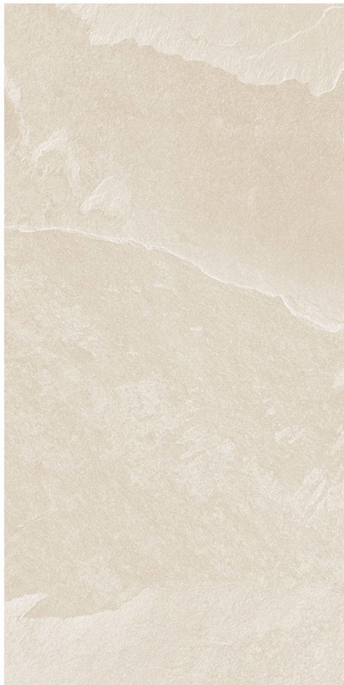
Random Design
