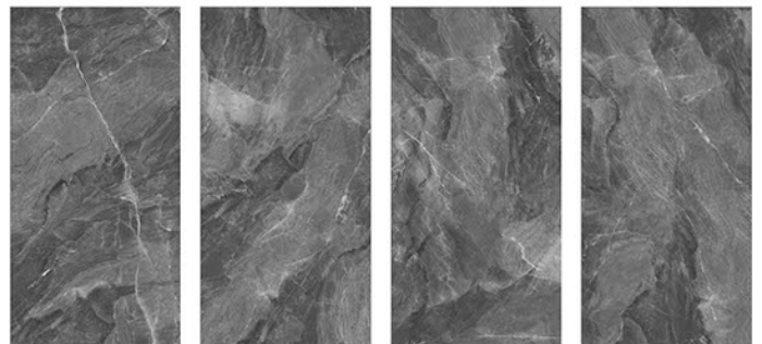
Random Design
